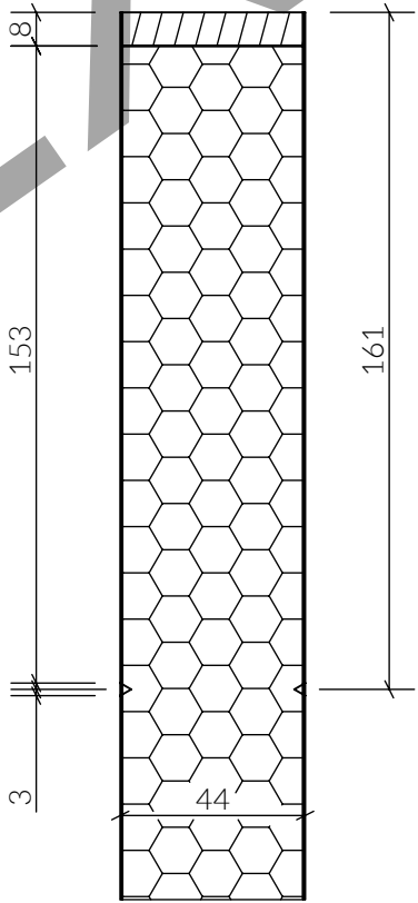
DETAIL M SCALE 1:2
