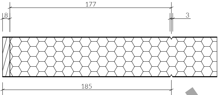
DETAIL N SCALE 1:2
