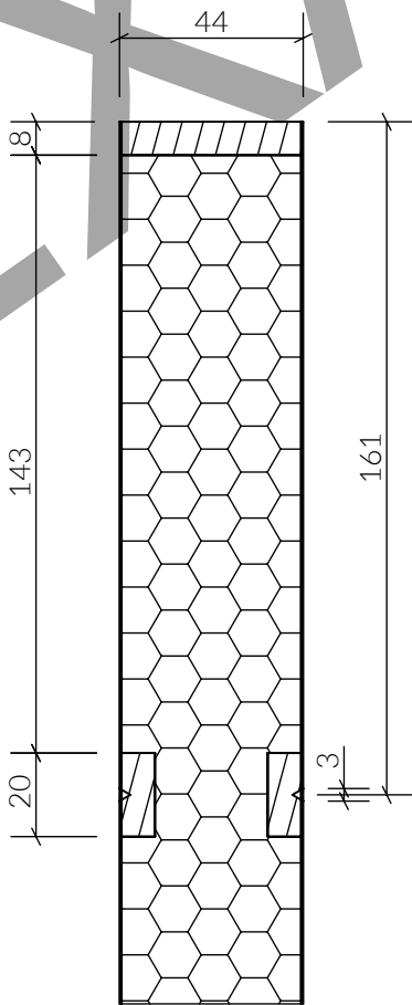
DETAIL M SCALE 1:2
