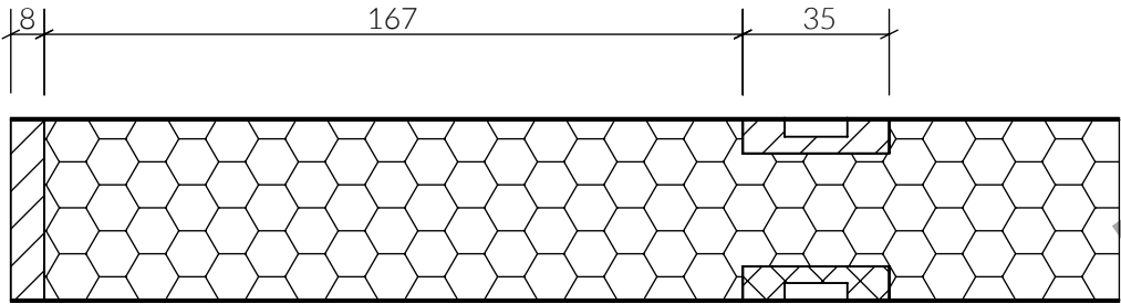
DETAIL N SCALE 1:2
