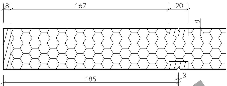
DETAIL N SCALE 1:2
