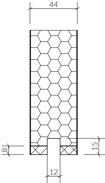
DETAIL K SCALE 1 : 2
