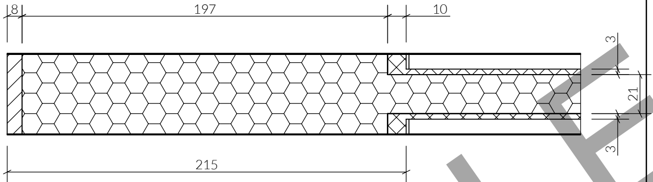
DETAIL N SCALE 1:2
