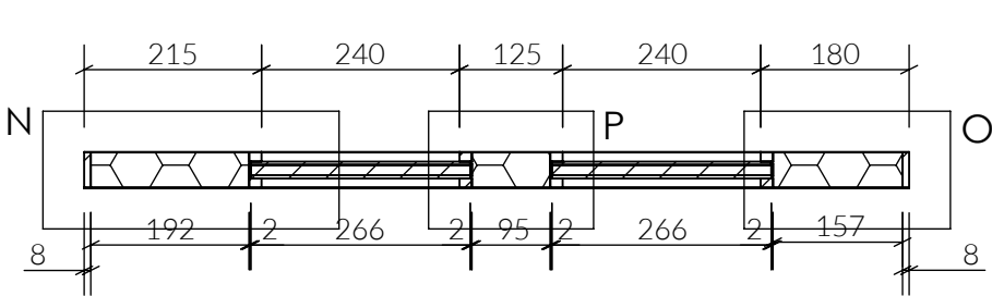
SECTION A-A SCALE 1:10
